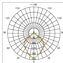
MQTL1223-10W
