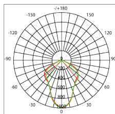
MQTL1223-20W
