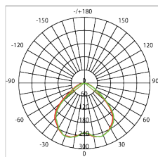
MQTL1223-7W
