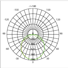
MXTL1045-30W
