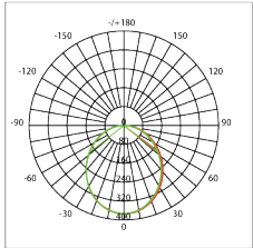
MXTL1045-12W
