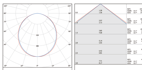
MQTL1241-12W
