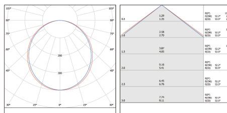
MQTL1241-15W
