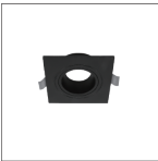
Size:92*92*30mm Cut-out:75*75mm
