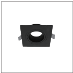
Size:92*92*30mm Cut-out:75*75mm
