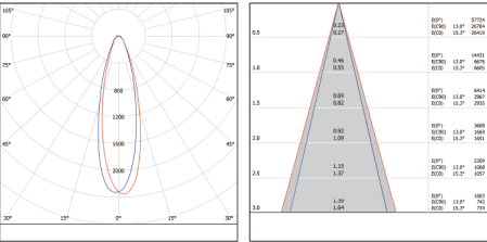
MDL1010-30W
