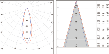
MDL1010-60W
